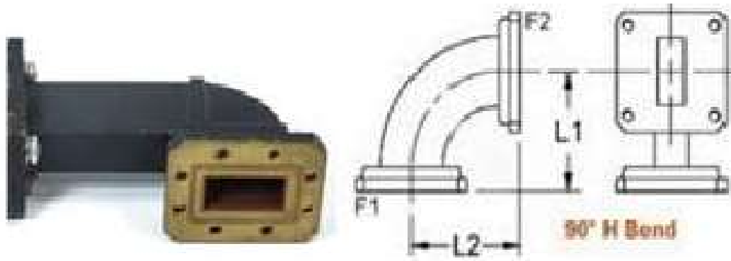
WR137 H Bend 2 x 4 CPRG/CPRF
