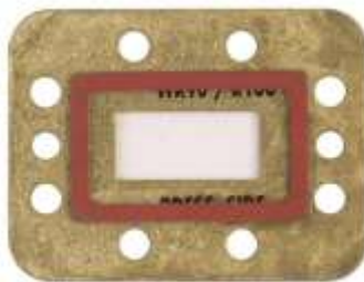
Pressure Window for WR137, 5.85–8.2 GHz, mates to CPR1
